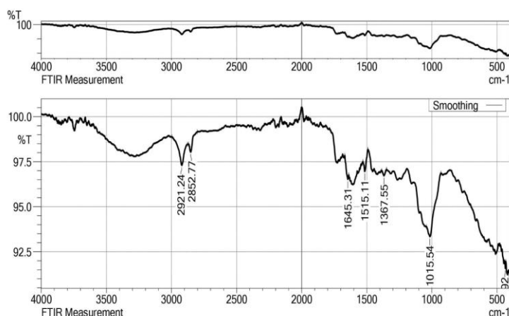
Figure No: 3 FT IR Analysis of Citrus limetta peel powder
