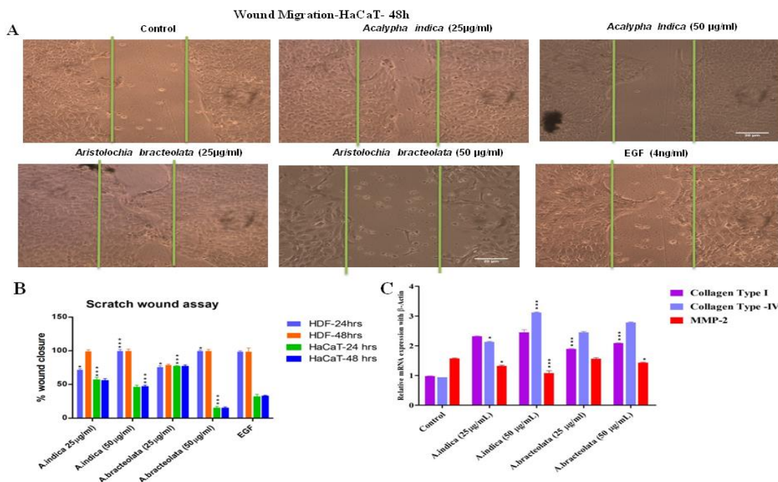
Figure 3: A)Phase contrast images of scratch wound assay on HaCaT cells after 24 & 48hrs. B) Graphical representation of rate of wound closure . Magnification – 20X. C) Analysis of mRNA expression of remodelling enzymes, extracellular matrix components associated with wound repair by RT-PCR analysis
