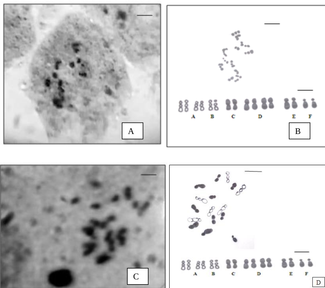
Figure 2: Photographs of metaphase plate, drawing and karyotype analysis from in vivo root (A-C) and callus (D-F) (Bar= 5μm).
