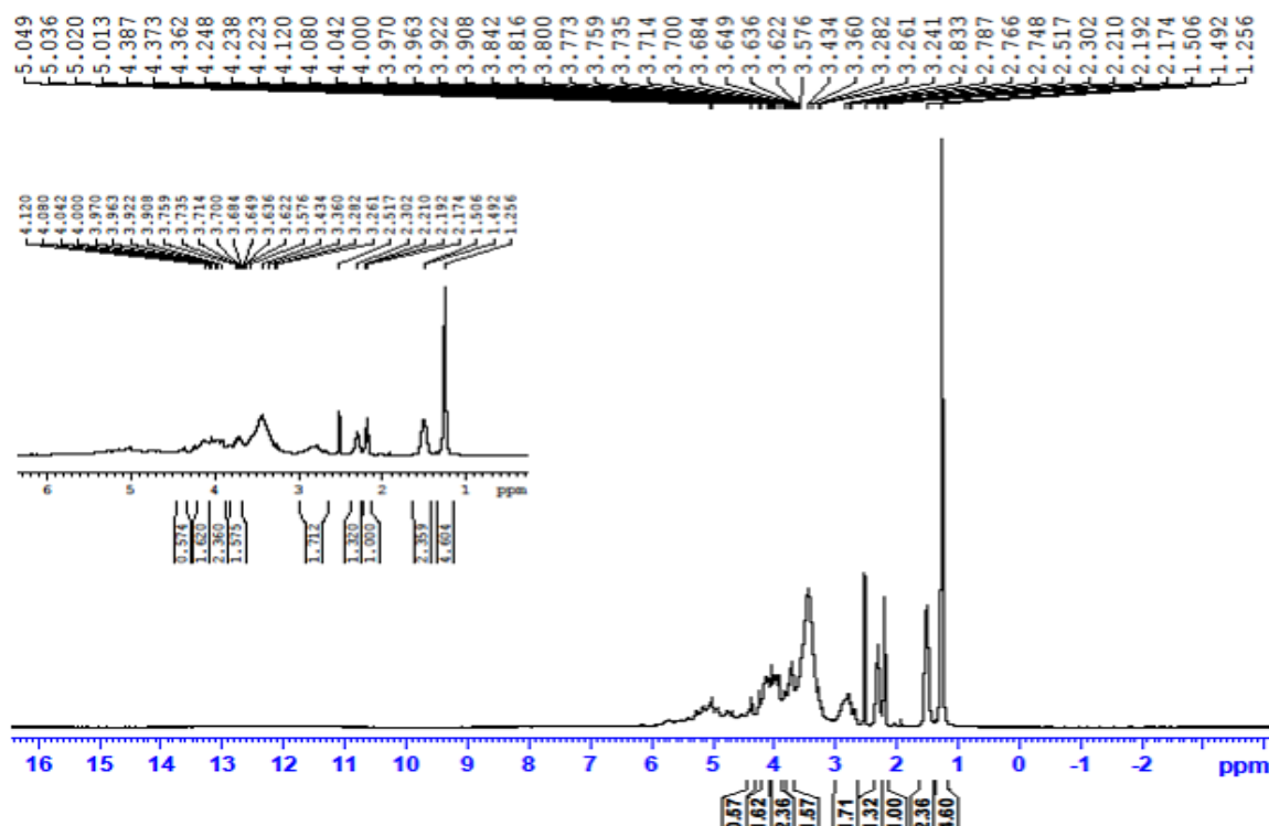
Fig.4.2 (c) ^1\text{H} NMR Spectrum of PSSC
