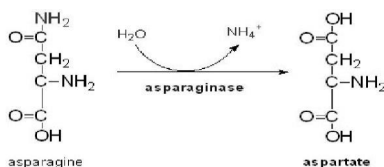
Fig 1 Hydrolysis of L-asparagine to aspartic acid and ammonia
