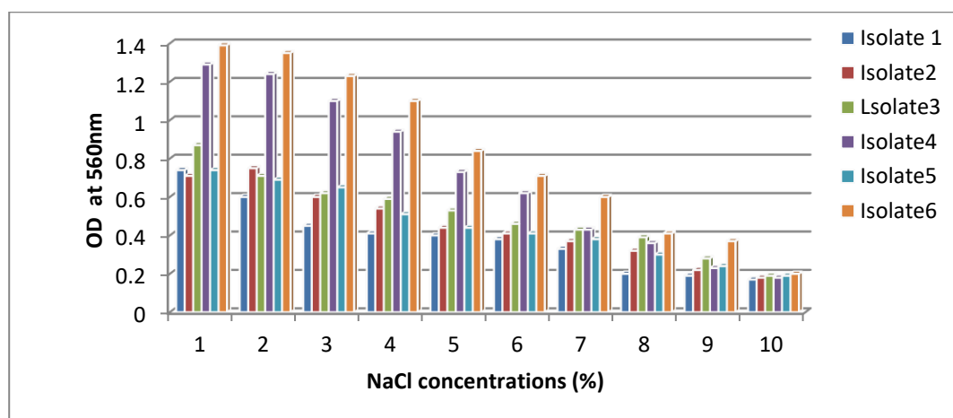
Figure 2 – Effect of NaCl concentration on the growth of isolated LAB.
