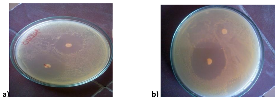
Figure- 4 (a, b) Zone of inhibition shown by isolated LAB against different pathogens
