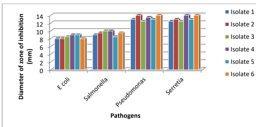
Figure 6 - Antimicrobial activity of isolated LAB
