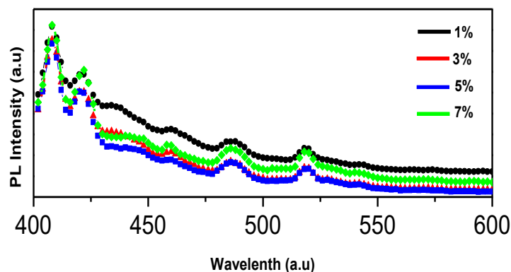
Figure 14(a-d) Photoluminescence patterns of Gd doped ZnSe thin films 500 °C with different mole concentration at (a) 1%, (b) 3%, (c) 5%, and (d) 7%.
