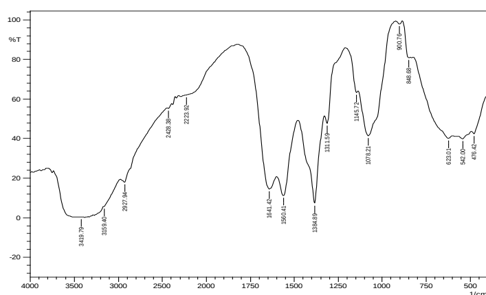
Figure 1: FT-IR spectrum of Pure COS
