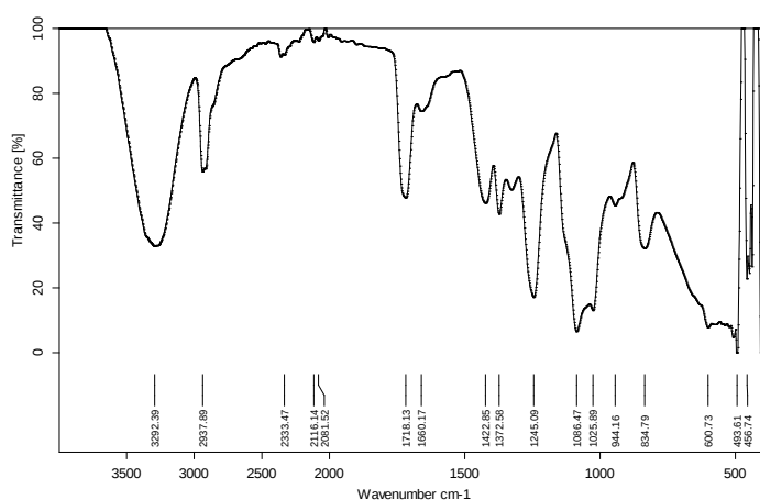
Figure 2: FT-IR spectrum of COS/PPG/MMT-GLU
