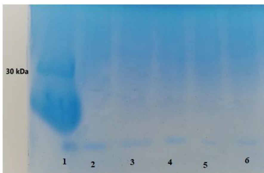
Figure 6: SDS-PAGE pattern of SEC fractions (7-11) by using 20 % resolving gel
