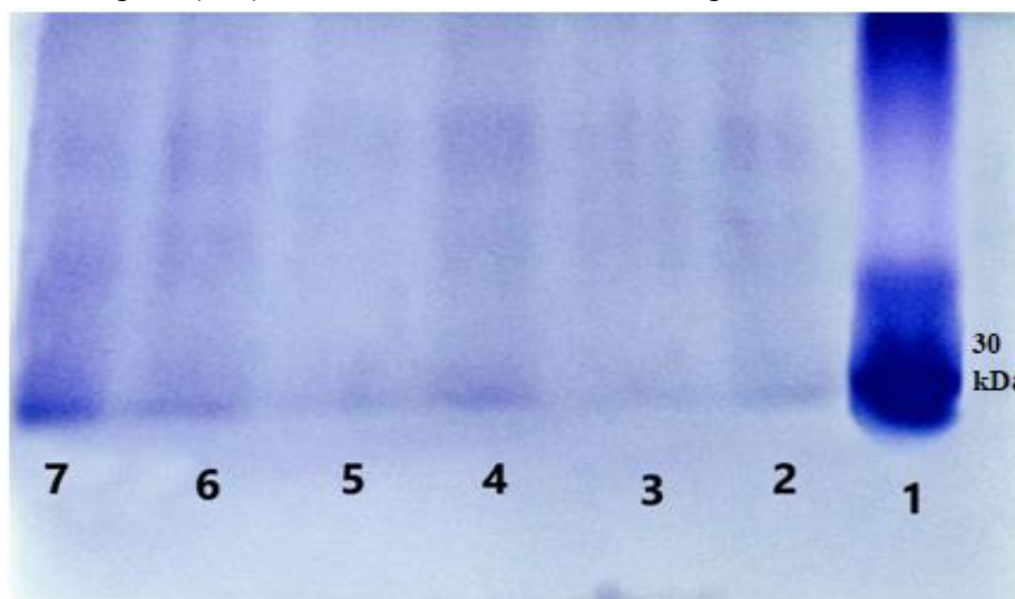
Figure 5: SDS-PAGE pattern of SEC fractions (1-6) by using 15 % resolving gel
