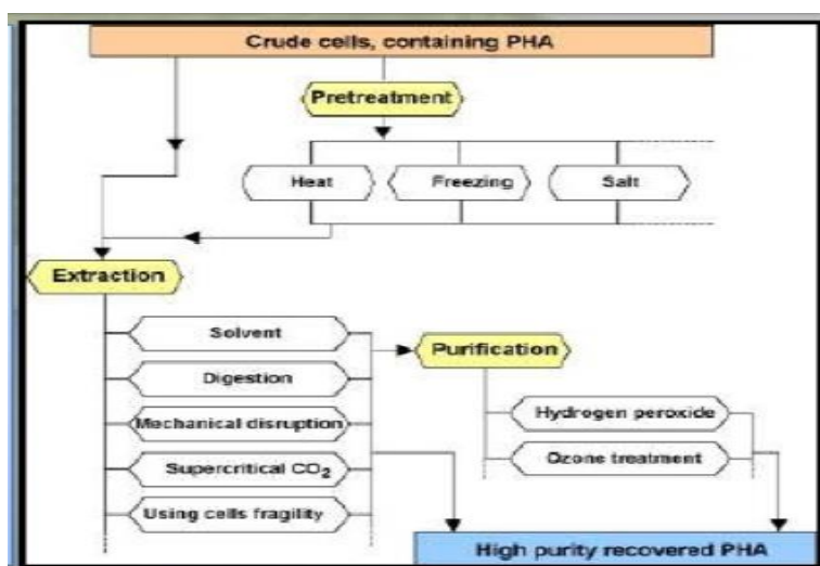
Fig 3: Extraction and Purification of PHA
