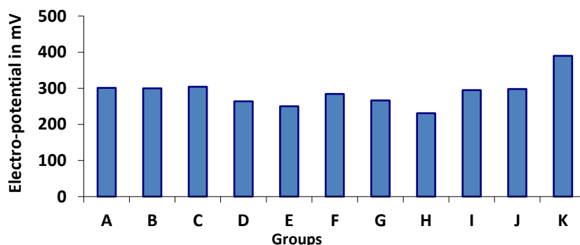
Fig. 2 Establishment of consortia
