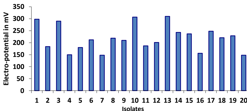
Fig. 1 Electro potentials generated by primary inoculants
