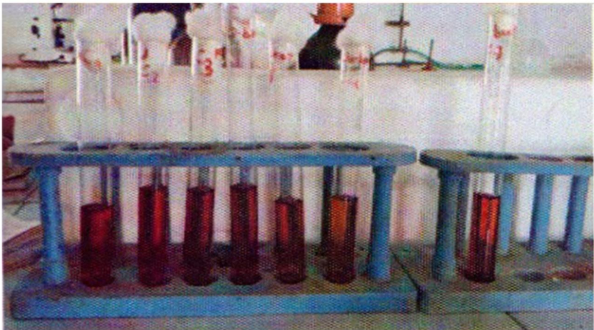
Biochemical test : Urea utilization
