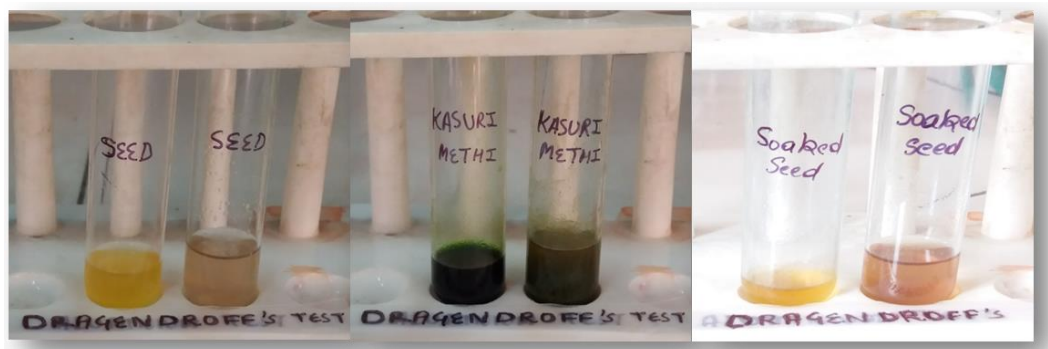
Figure 6: Dragendorff's test
