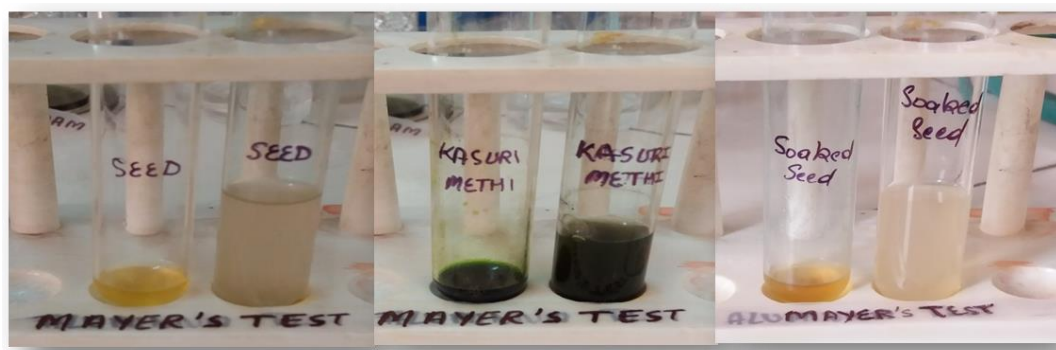
Figure 7: Mayer's test
