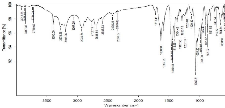
Fig 3: FTIR Spectrum of Formulation F4
