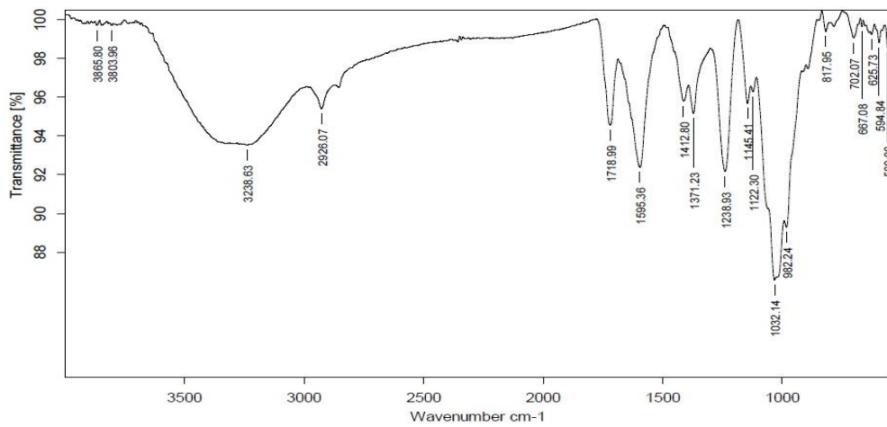
Fig 2: FTIR Spectrum of Almond gum
