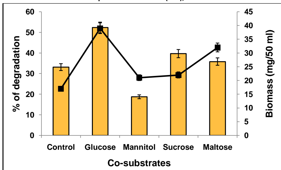
Figure 2: Effect of co-substrates on BaP degradation and fungal biomass production. Data represent mean ± S.D. (n=3); P < 0.05
