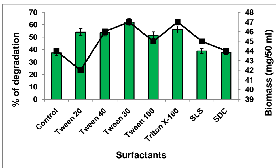
Figure 4: Effect of surfactants on BaP degradation and fungal biomass production. Data represent mean \pm S.D. (n=3); P < 0.05
