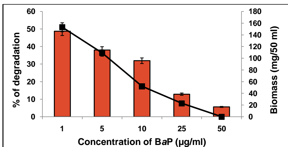
Figure 1: Effect of BaP concentration on its degradation and fungal biomass production. Data represent mean ± S.D. (n=3); P < 0.05 .
