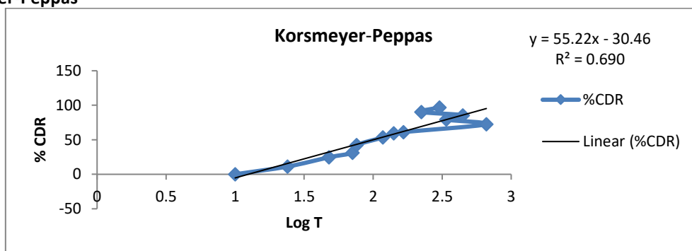
Fig-8: Korsmeyer-Peppas
