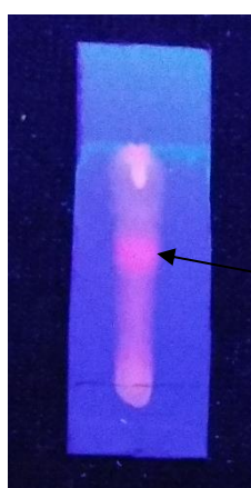
Fig 18: Thin layer chromatography of parthenin
