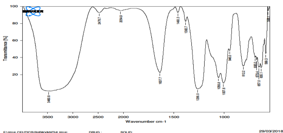
FTIR Spectrums of drug and optimized form
