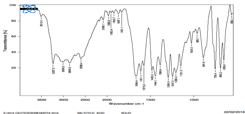
Figure 4: salicylic acid FTIR spectrum
