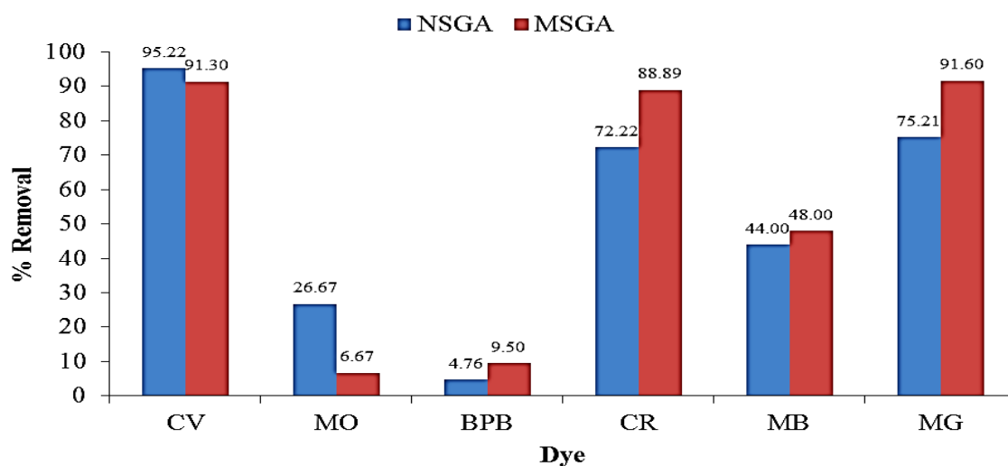
Figure 3: Comparison of % removal of six dyes by NSGA and MSGA after 120 min. (CV: Crystal Violet; MO: Methyl Orange; BPB: Bromophenol Blue; CR: Congo Red; MB: Methylene Blue; MG: Malachite Green)
