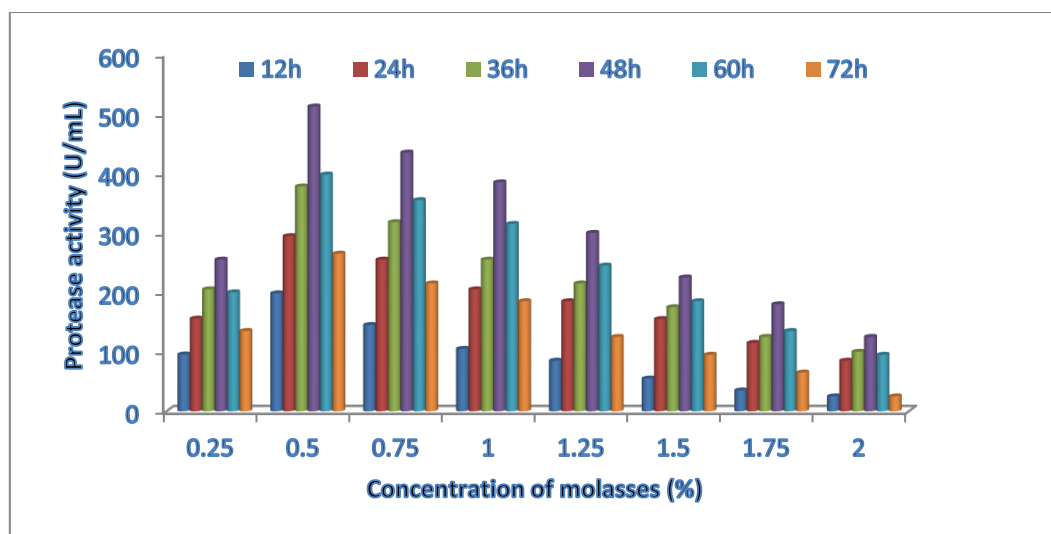
Fig. 9: Influence of different concentration of molasses on protease production.
