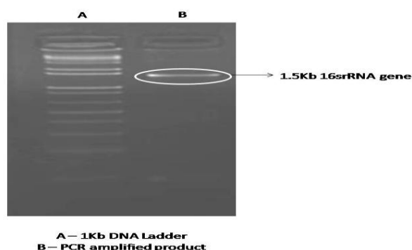
Fig.No.6 Gel picture depicting 16srRNA amplicon
