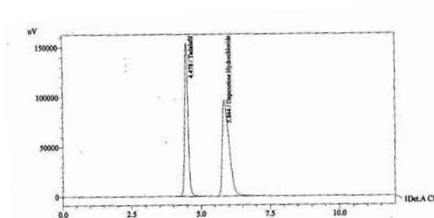
Figure 3 : Typical HPLC Chromatogram of Sample Tablets (Tadalafil and Dapoxetine hydrochloride)
