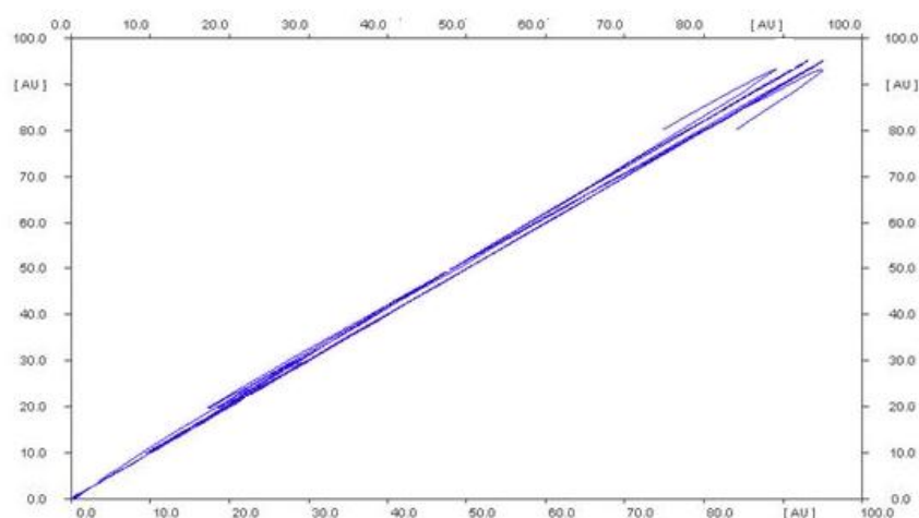
Figure 4: Peak purity spectra of Etravirine from tablet dosage form
