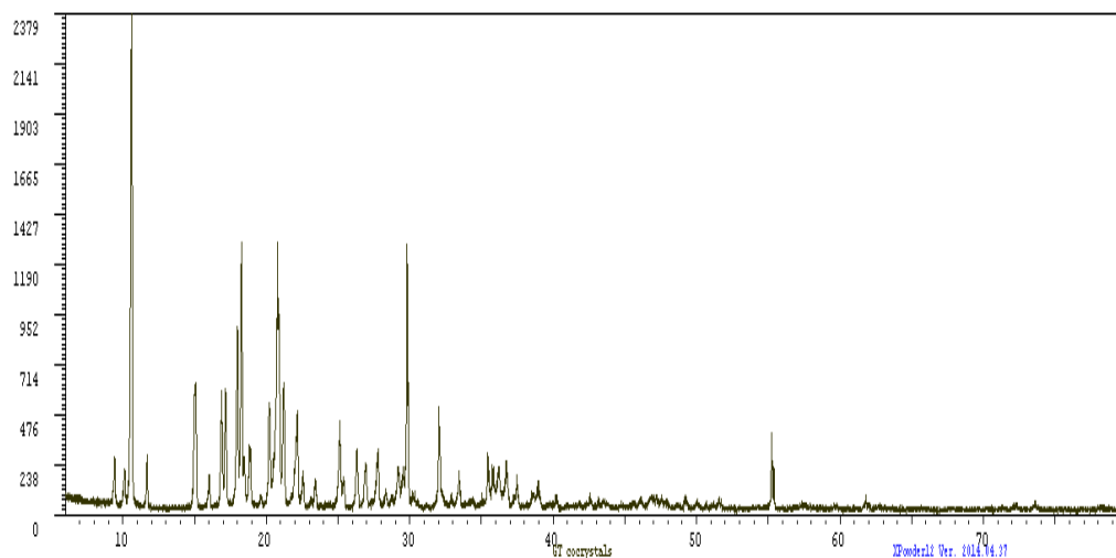
Fig No.10 Powder X-ray diffraction of gliclazide and Tartaric acid cocrystals
