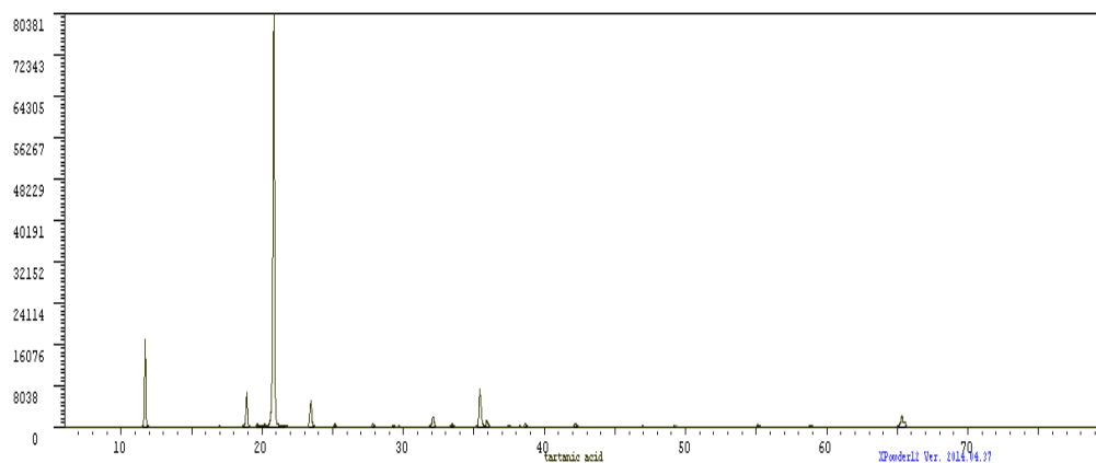
Fig No.9 Powder X-ray diffraction of Tartaric acid
