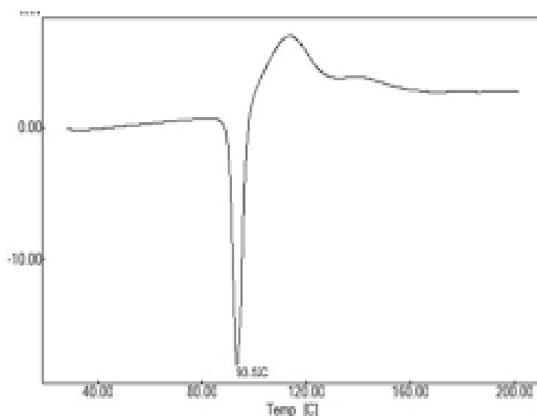
Fig no.6 Differential scanning calorimetry of tartaric acid
