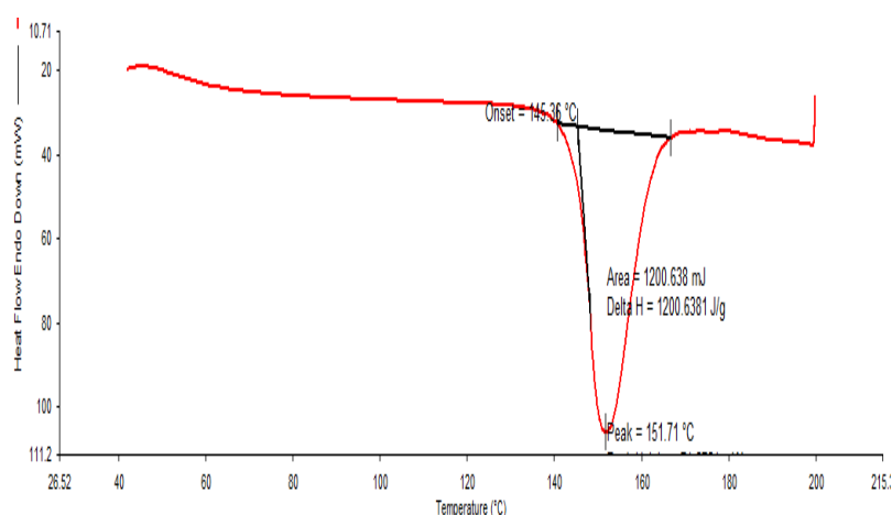
Fig.No.7 DSC thermogram of gliclazide and tartaric acid cocrystals
