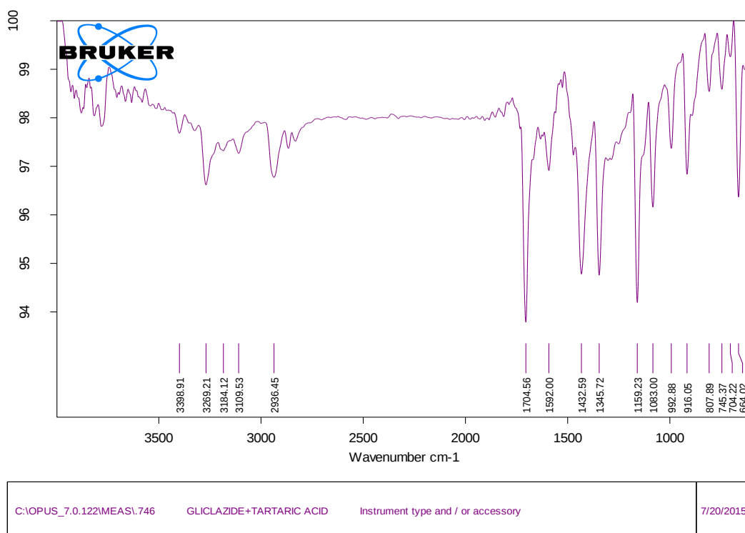
Fig No.4 FTIR characteristic peaks of gliclazide and tartaric acid cocrystals
