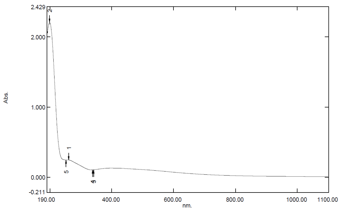
Fig.6: UV –vis spectrum of the Ag NPs synthesized using SAECE extract
