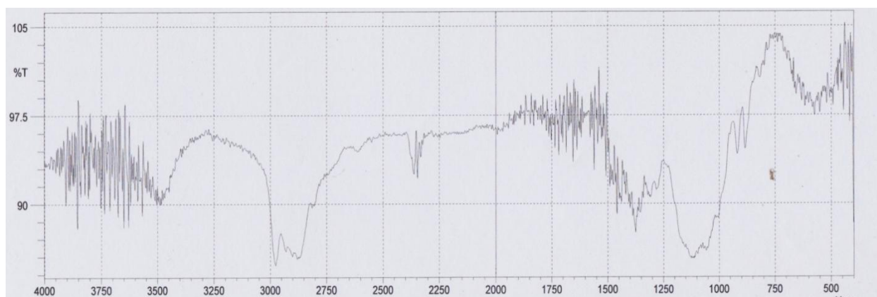
Fig.20: FTIR image of Ag NPs synthesized using SAEAC extract
