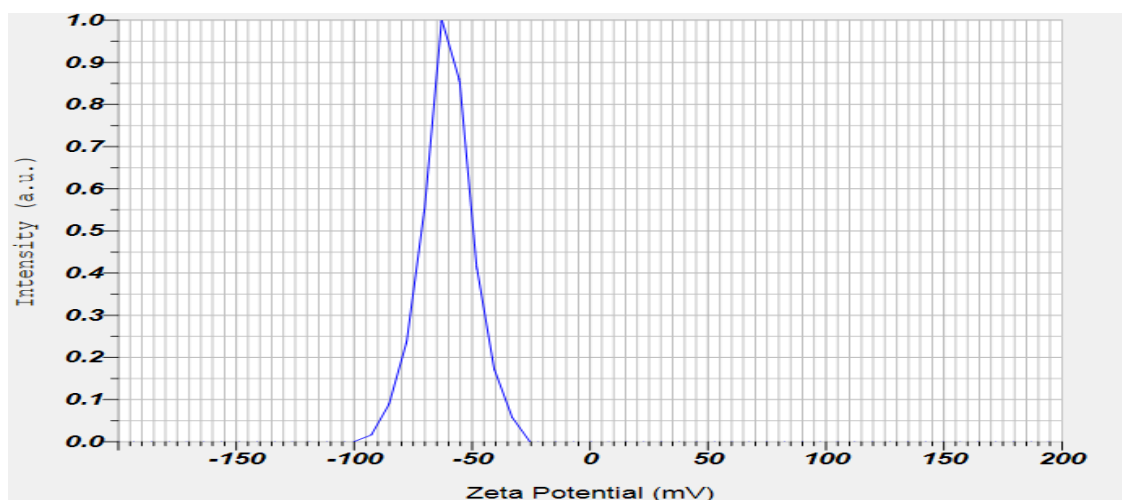
Fig.11: The Zeta potential value of dispersed biosynthesized Ag NPs of SAEAPE was found to be -60.5mV, typically have degree of stability.
