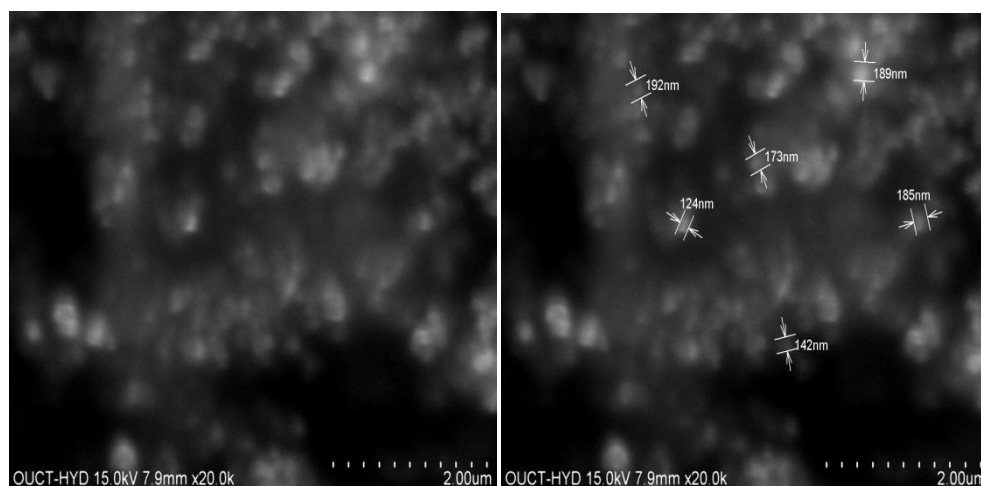
Fig.15: SEM image of Ag NPs synthesized using SAEAP extract
