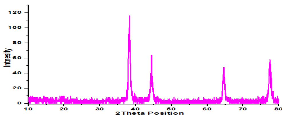
Fig.17: XRD image of Ag NPs synthesized using SAEAP extract
