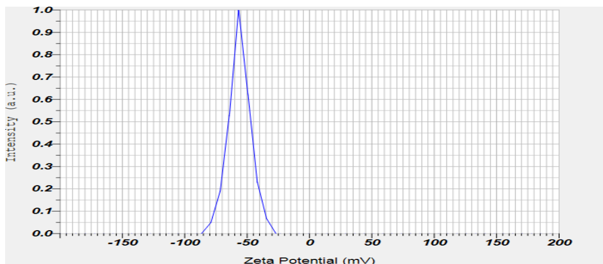
Fig.12: The Zeta potential value of dispersed biosynthesized Ag NPs of SAEACE was found to be -56.1 mV, typically have degree of stability.
