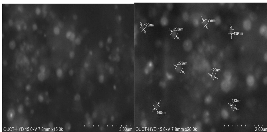
Fig.16: SEM image of Ag NPs synthesized using SAEAC extract
