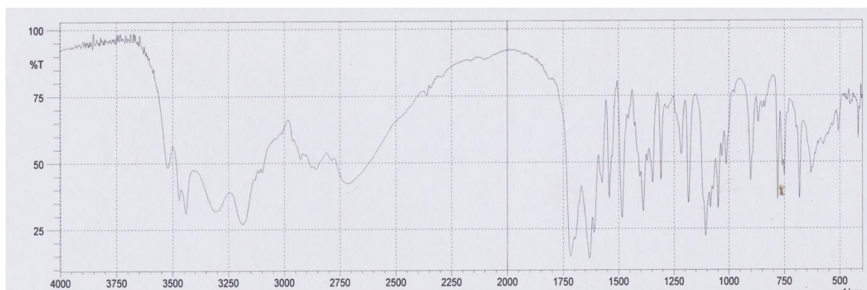
Fig.19: FTIR image of Ag NPs synthesized using SAEAP extract
