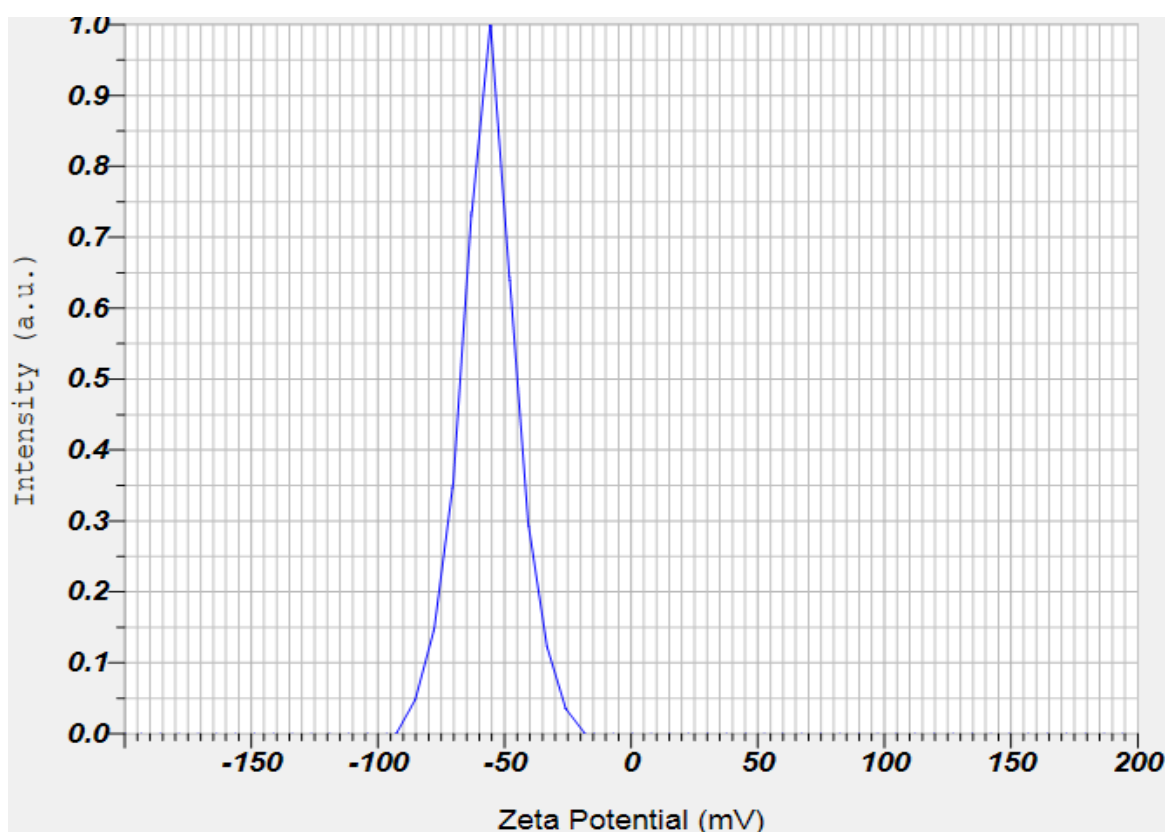
Fig10: The Zeta potential value of dispersed biosynthesized Ag NPs of SAECE was found to be -56.3mV, typically have degree of stability.
