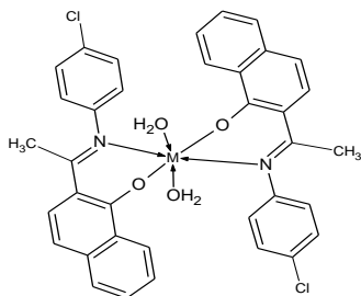
Figure 3. The metal-ligand binary binding proposed structure.
