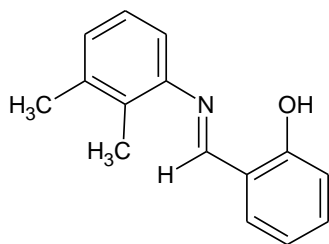
Figure 1. Primary ligand 2-[(E)-[(2,3-dimethylphenyl) imino] methyl} phenol
