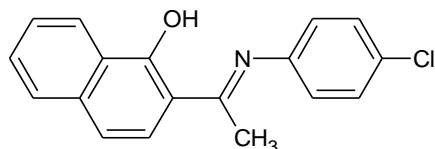
Figure 2. Secondary ligand 2-[(1E)-N-(4-chlorophenyl) ethanimidoyl] naphthalen-1-ol
