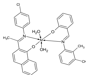
Figure 4. The metal-ligand ternary binding proposed structure.
