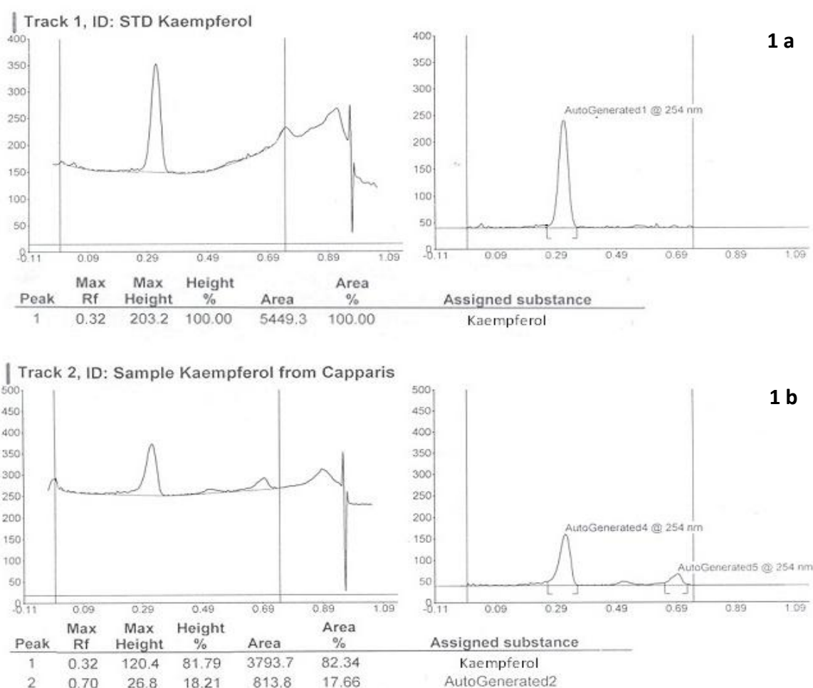
Figure 1: HPTLC chromatogram of (a) Std. kaempferol and (b) Isolated kaempferol in solvent system benzene: acetic acid: water (125:72:3) scanned at 254 nm
