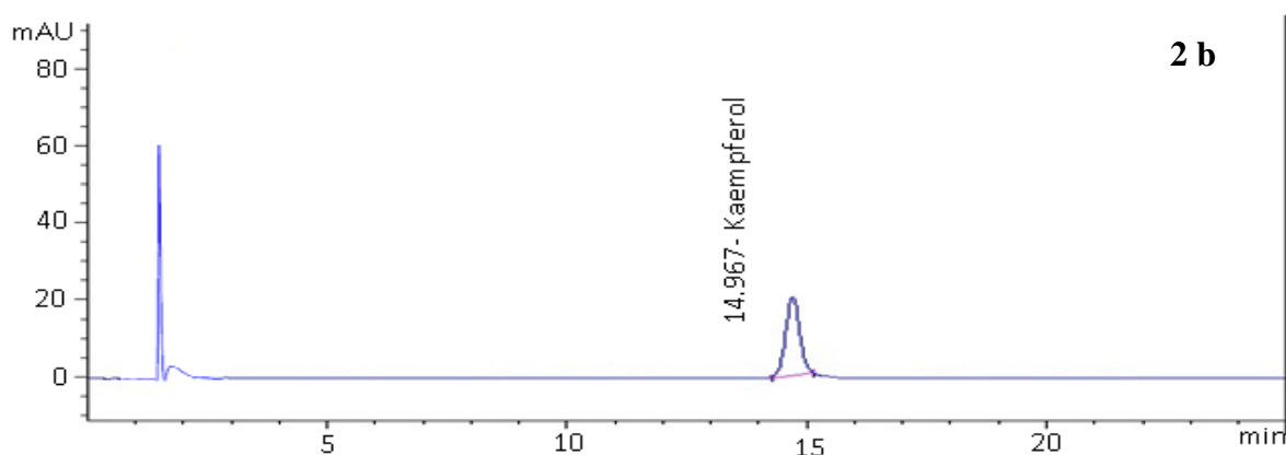
Figure 2: HPLC chromatogram of (a) Std. kaempferol and (b) Isolated kaempferol in mobile phase solution A (water: orthophosphoric acid, pH 3.0) and solution B (acetonitrile: methanol in ratio of 75:25) (50:50) scanned at 370 nm
