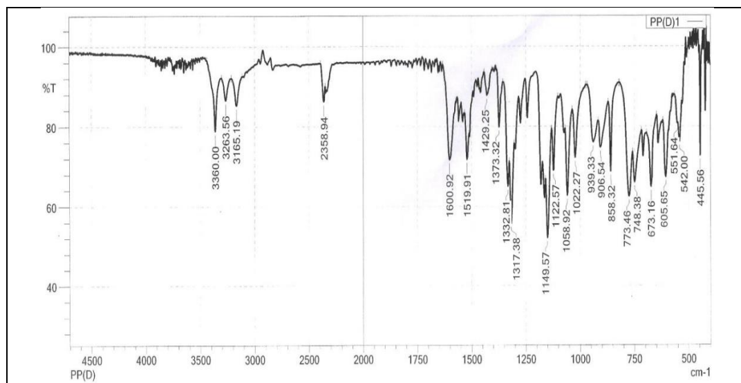
Figure 15: ATR spectra of Hydrochlorothiazide
