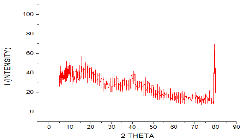
Figure.No 8 : [\text{Rh}(\text{HL})\text{Cl}_3\text{H}_2\text{O}]\cdot 2\text{H}_2\text{O}
