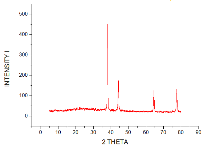
Figure.No.9 : [\text{Pt}(\text{HL})\text{Cl}_2]\text{H}_2\text{O}
