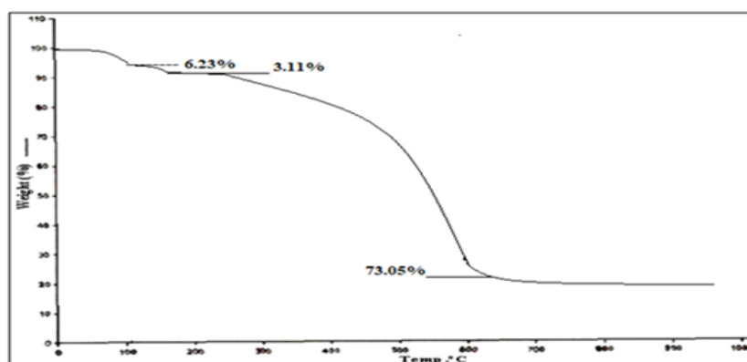
Figure.No 1 : TGA of [\text{Rh}(\text{HL})\text{Cl}_3\text{H}_2\text{O}]\cdot 2\text{H}_2\text{O}
