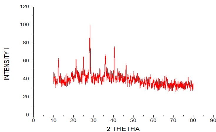
Figure.No.9 : [\text{Pt}(\text{HL})\text{Cl}_2]\text{H}_2\text{O}
