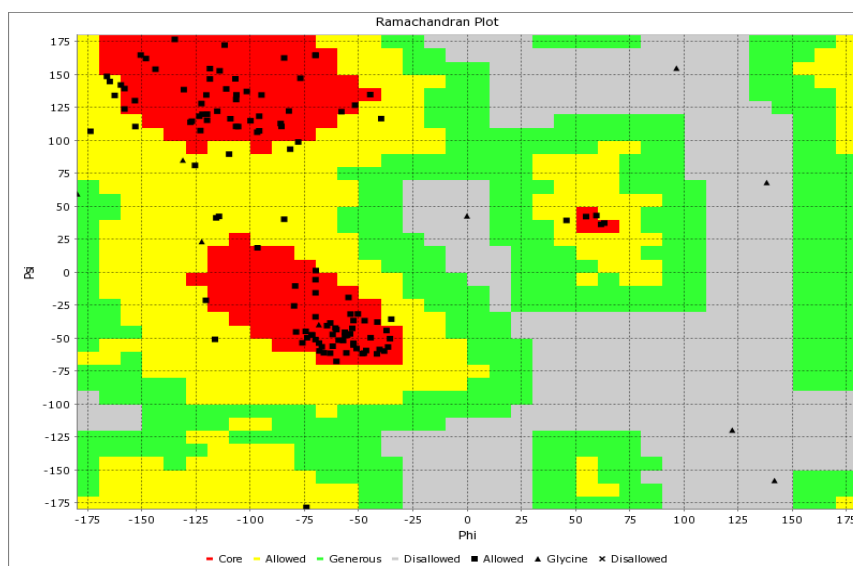
Fig. 3. Ramachandran plot
