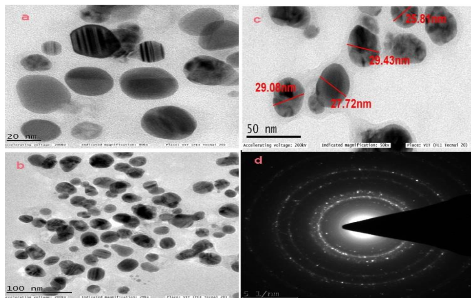
Fig. 5 TEM Images: a) Spherule shape of SNPs at 20 nm, b). Dispersion of the nanoparticles at 100 nm, c). Average size of AgNPs at 50 nm 28.01nm and d). Imaging at 51 nm.
