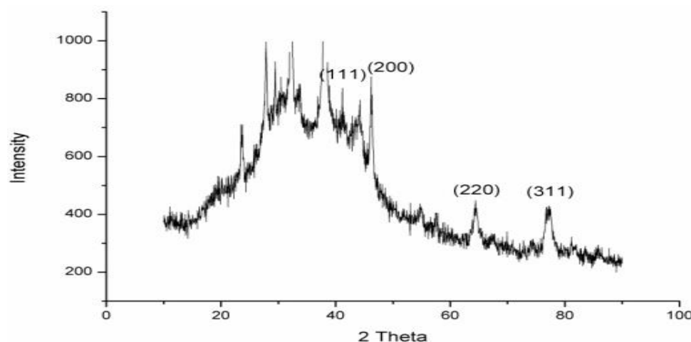
Fig. 6 XRD pattern of AgNPs shows Bragg reflections
