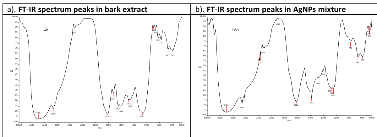
Fig 2 a) Walsura trifoliata bark - FT-IR spectrum peaks in bark extract and b) BV1 - FT-IR spectrum peaks in SNPs mixture.
