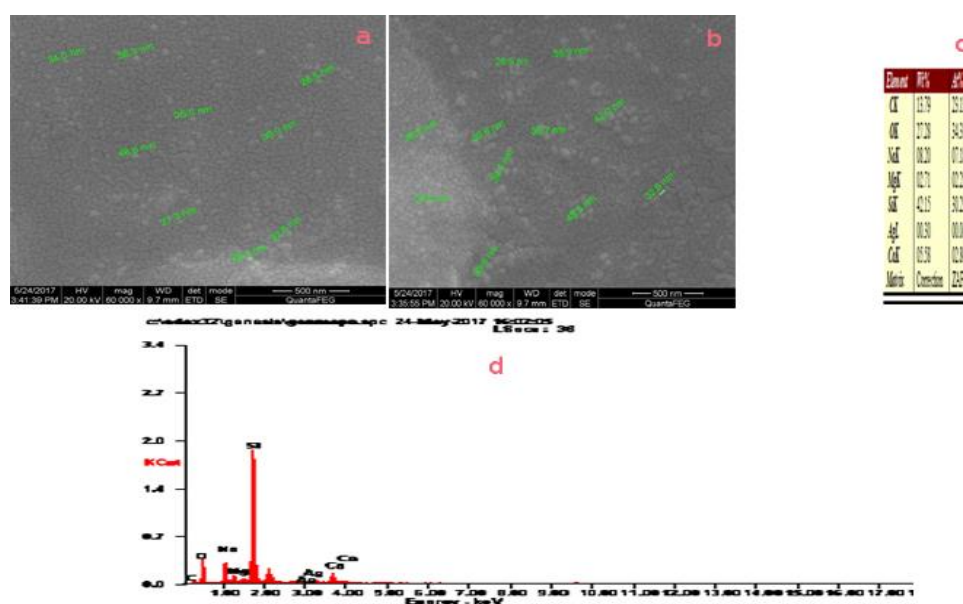
Fig. 4 SEM images: a) and b) average size of the AgNPs 33.85nm from Walsura trifoliata Stem bark from Walsura trifoliata bark, c) and d) EDAX analysis in the weight percentage of silver in mixture.
