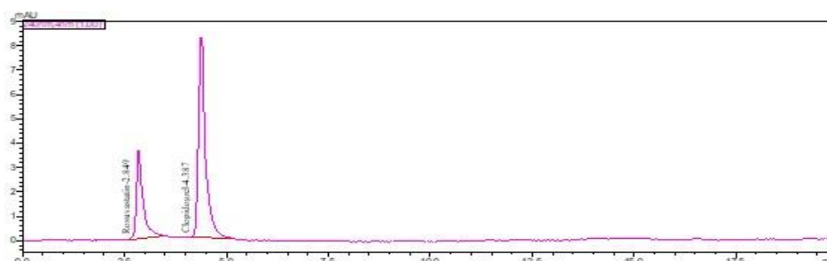
Figure 6: A typical chromatograph of mixture of sample RSV and CLO Rosuvastatin calcium (RSV) and Clopidogrel bisulfate (CLO) with Rt of 2.849 min. and 4.387 min. respectively.
