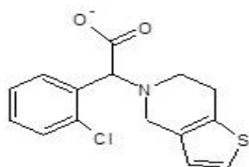
Figure 2: Chemical structure of clopidogrel bisulfate (CLO)
