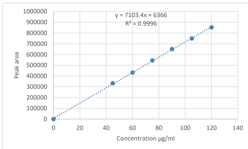
Figure 4: Linear curve clopidogrel bisulfate (CLO)
