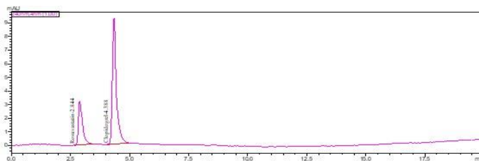
Figure 5: A typical chromatograph of mixture of standard RSV and CLO Rosuvastatin calcium (RSV) and Clopidogrel bisulfate (CLO) with Rt of 2.844 min. and 4.388 min. respectively.
