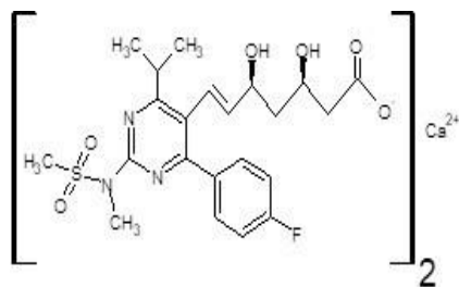
Figure 1: Chemical structure of rosuvastatin calcium (RSV)
