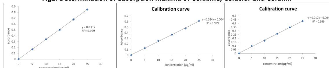
Fig3: Standard curve of CEFIXIME, CEFACTOR and CEFDINIR in pH 6.8(λ max 286, 268 and 282nm)
