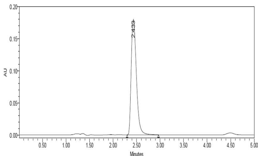
Figure 2: typical chromatogram of by proposed method
