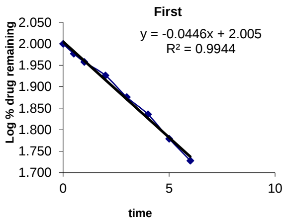
Fig 13: First order release kinetics graph
