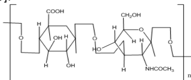
Fig-4: Structure of Hyaluronic acid
