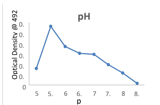
Figure.8. Effect of pH on growth
