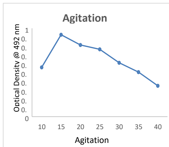
Figure.10. Effect of Agitation speed on growth
