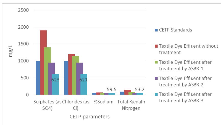
Figure 6 Comparison of CETP standard with effluents treated by ASBR's results-Graph 2
