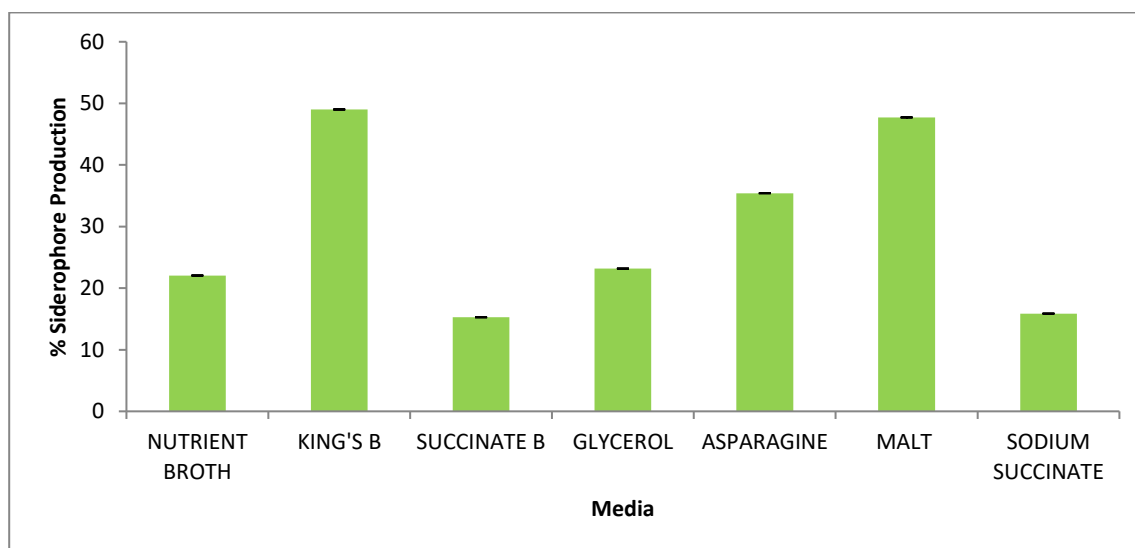
Fig.2: Effect of different media on siderophore production
