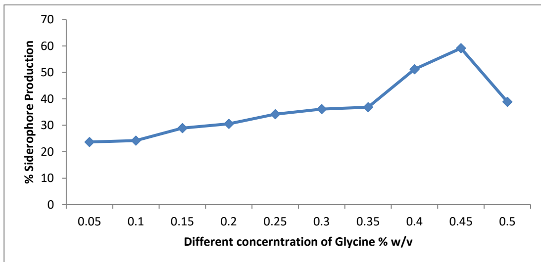
Fig.13: Effect of various concentration of glycine in King's B medium on siderophore production
