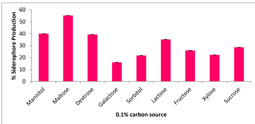
Fig.10: Effect of different carbon sources on siderophore production
