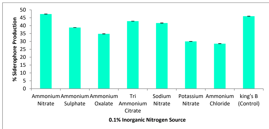
Fig. 14: Effect of different Inorganic Nitrogen Source on siderophore production
