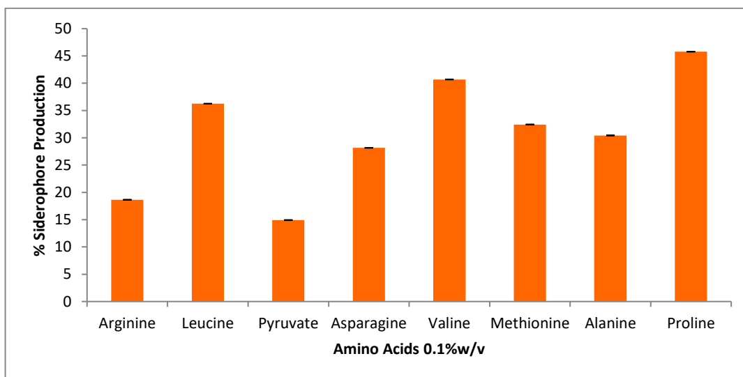
Fig.16: Effect of different amino acids on siderophore production
