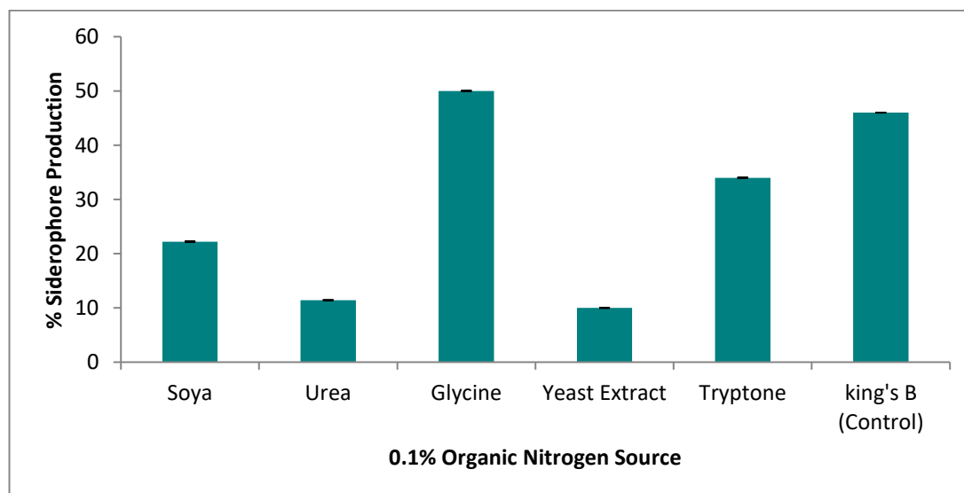
Fig.12: Effect different Organic Nitrogen Source on siderophore production
