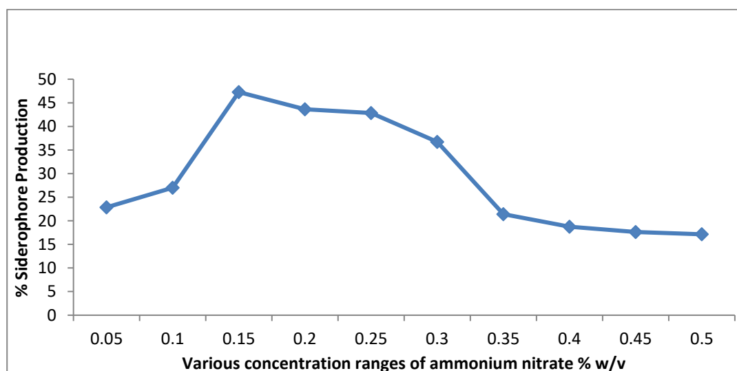
Fig.15: Effect of Different concentration range of Ammonium Nitrate on siderophore production
