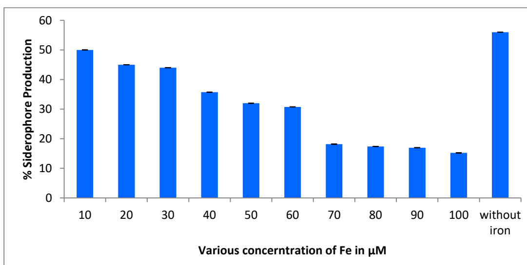
Fig.9: Effect of Different Iron concentration on siderophore production
