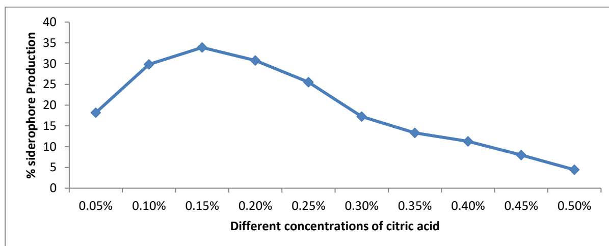
Fig.19: Effect of Different concentration of citric acid on siderophore production
