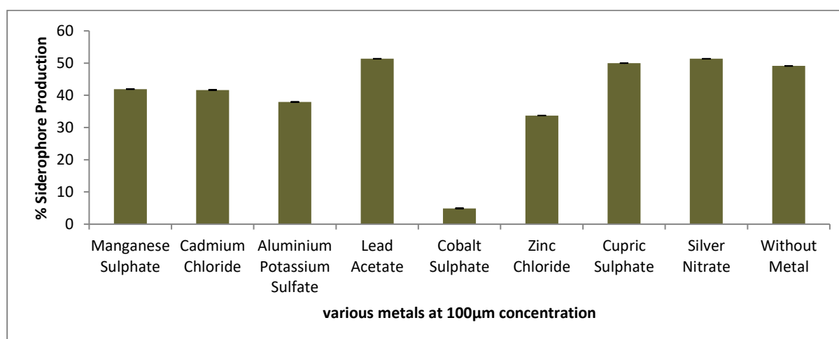
Fig.20: Effect of different metals on Siderophore Production
