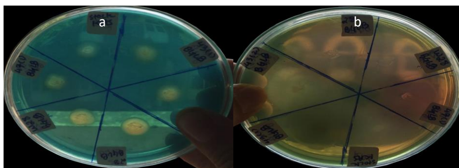
Fig.1: Qualitative screening of siderophore production by using CAS agar plates. Light orange yellow hallos observed on day 1 (a) and day 5 (b)
