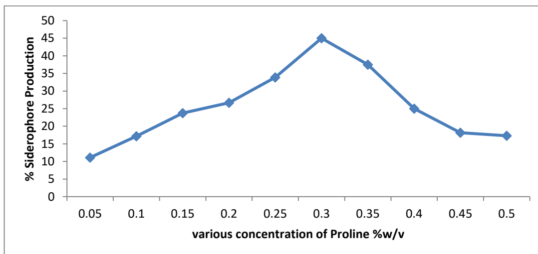
Fig.17: Effect of different concentration range of proline on siderophore production
