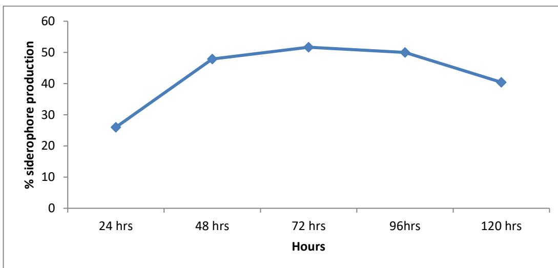
Fig.4: Effect of incubation time on siderophore production
