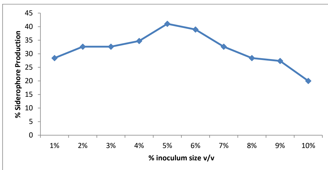
Fig. 5: Effect of inoculum size on siderophore production
