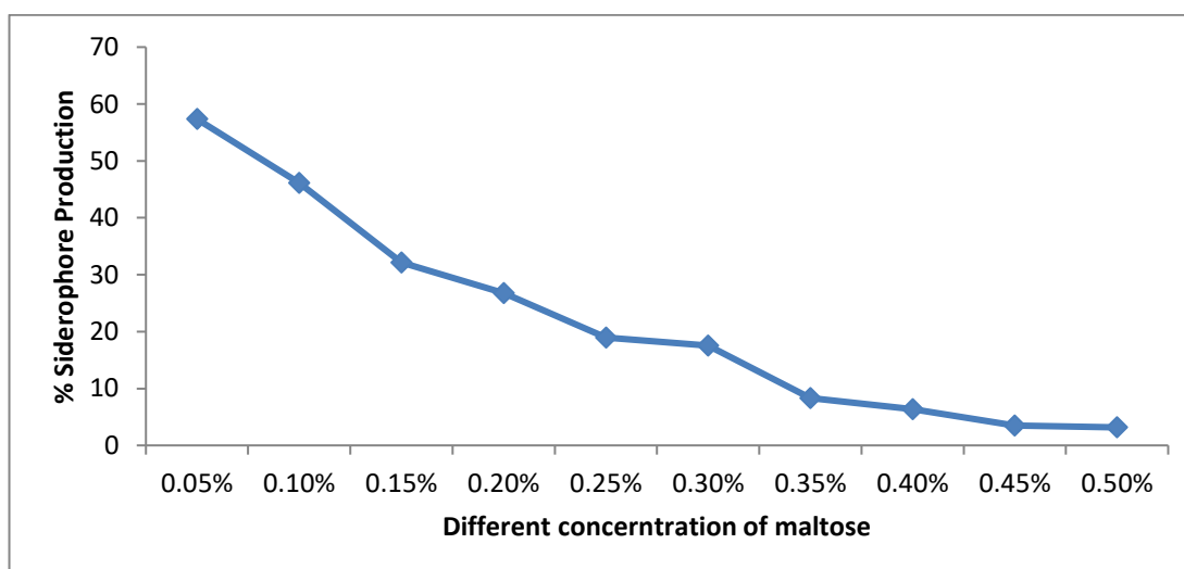
Fig. 11: Effect of various concentrations of maltose on siderophore production
