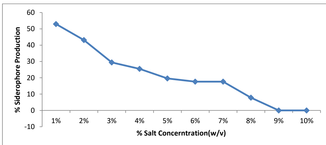
Fig. 8: Effect of NaCl on siderophore production
