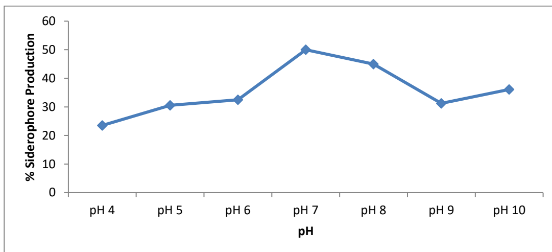
Fig. 7: Effect of pH on siderophore production
