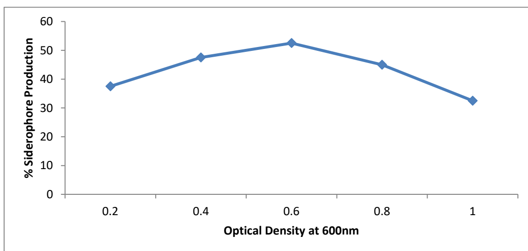
Fig.6: Effect of optical density on siderophore production
