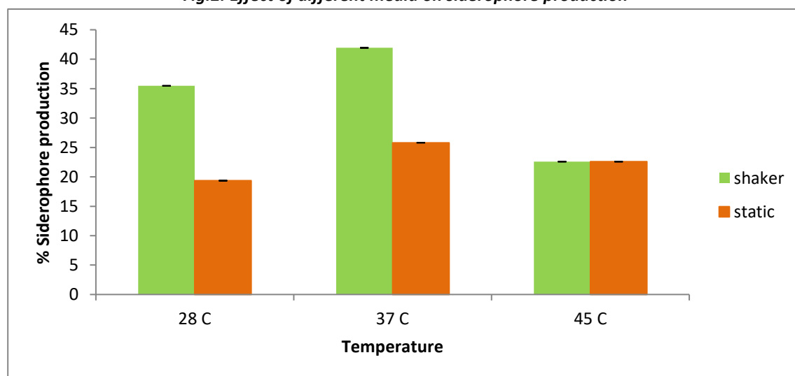
Fig.3: Effect of temperature and aeration on siderophore production
