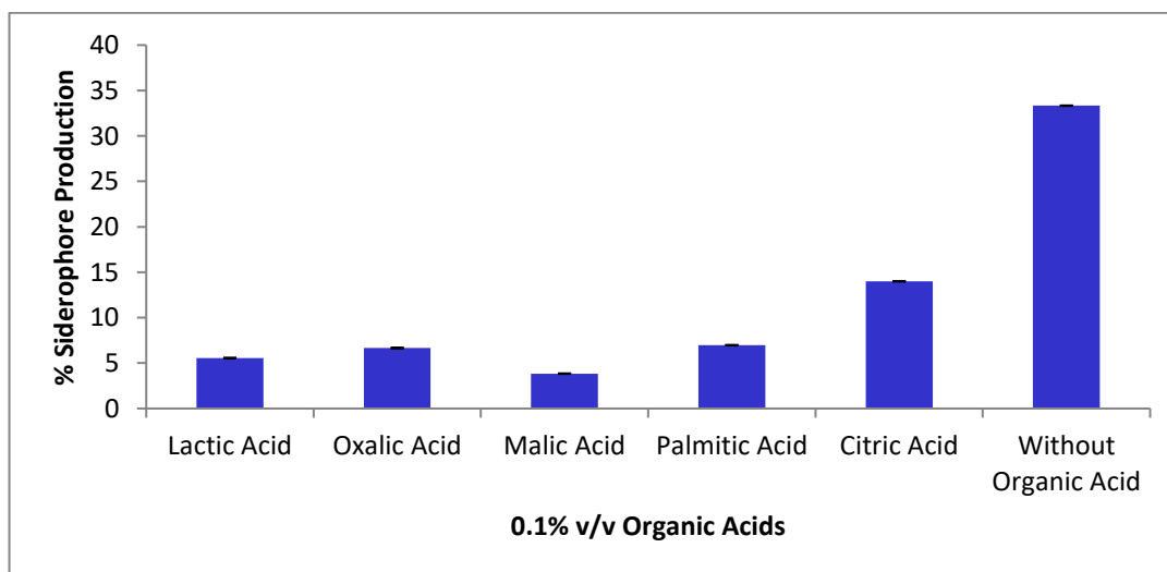
Fig.18: Effect of various Organic acids on siderophore production
