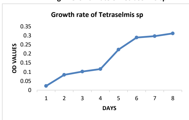
Fig.1. Growth rate of Tetraselmis sp.
