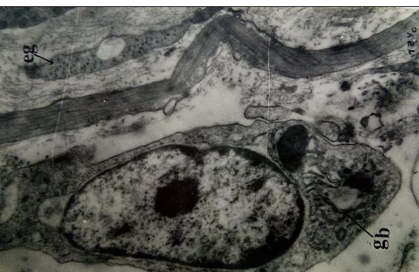
Figure 4b: Electron micrograph of NS cells showing electron dense granules to one of the branches at axon terminal end; golgi complex seen at the apex of nucleus in non-neurosecretory neuron (x15000). [eg = electron dense granule, gb = golgi body]
