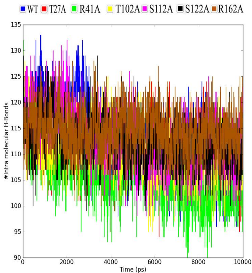
Figure 4: Total number of intra molecular hydrogen bonds graphs of the CD44 wild type protein compared with the mutant versions of the protein.
