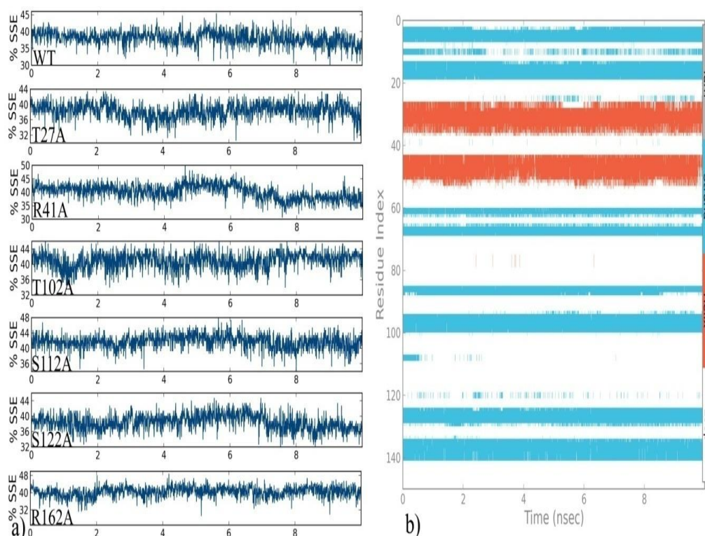
Figure 6: a) Secondary structure elements (SSE) graphs of the CD44 wild type protein compared with the mutant versions of the protein. b) Detailed Secondary structure elements (SSE) graph of T27A mutant version of CD44.
