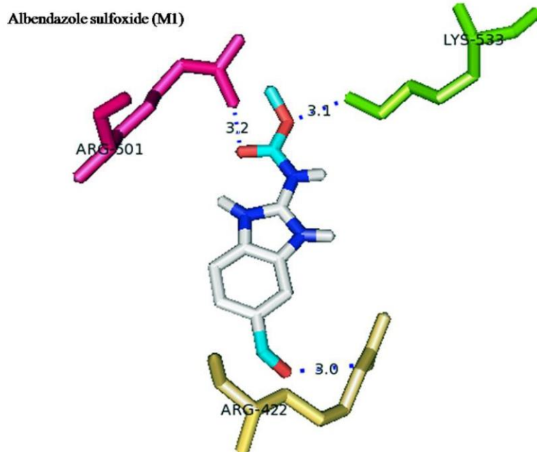
Fig.2 Snapshot of Albendazole sulfoxide (M1) and its hydrogen-bond interactions with 2GIR
