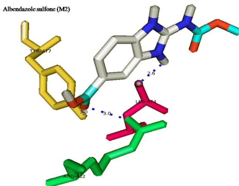
Fig.3 Snapshot of Albendazole sulfone (M2) and its hydrogen-bond interactions with 2GIR
