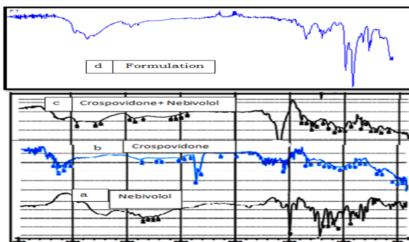
Figure 1: FTIR Spectra of (a) Nebivolol (b) crospovidone (c) Nebivolol + crospovidone (d) formulation
