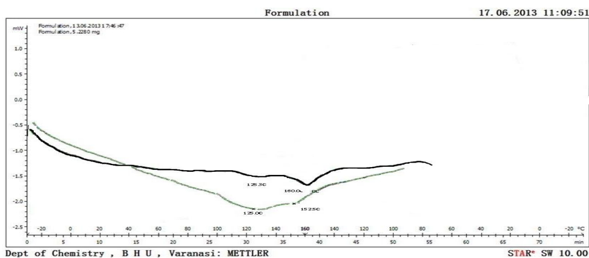
Figure 3: DSC curve of phytosomal formulation shown by black solid line and DSC curve of physical mixture of phosphatidylcholine and extract is shown by green solid line.
