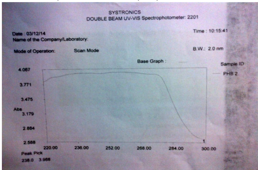
Graph 1: Double beam UV-VIS spectrophotometer
