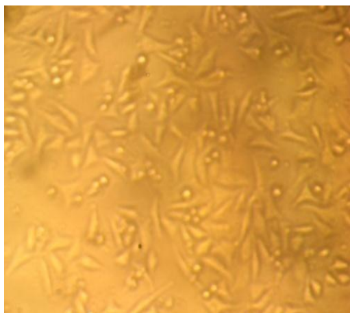
Toxicity 2 (62.5µg/ml)
