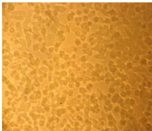
Toxicity 2 (500µg/ml)
