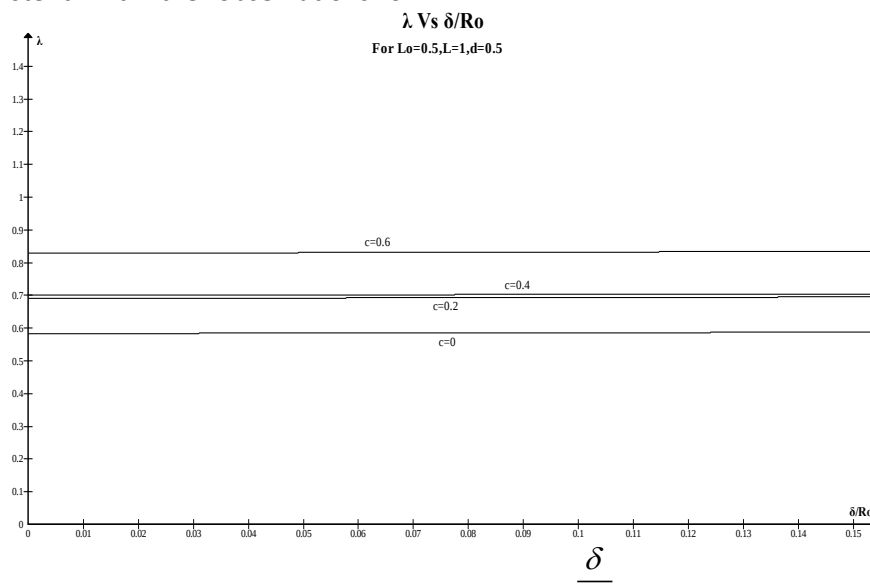
Figure 2 Variation of impedance, \lambda with \frac{\delta}{R_0} for different C
