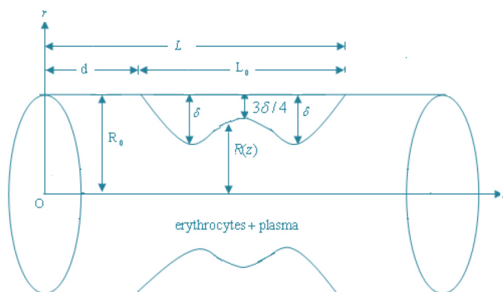
Figure 1 Geometry of an overlapping stenosis
