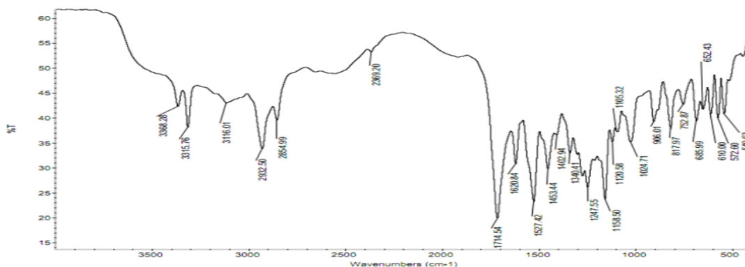
Figure 8: IR spectra of Glibenclamide + Carbopol 934P + Xanthan gum
