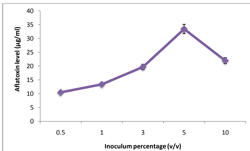
Figure 7: Effect of inoculum percentages on aflatoxin production from A. flavus MTCC 2798 in SmF. Data represents mean \pm S.D. (n=3); P < 0.05
